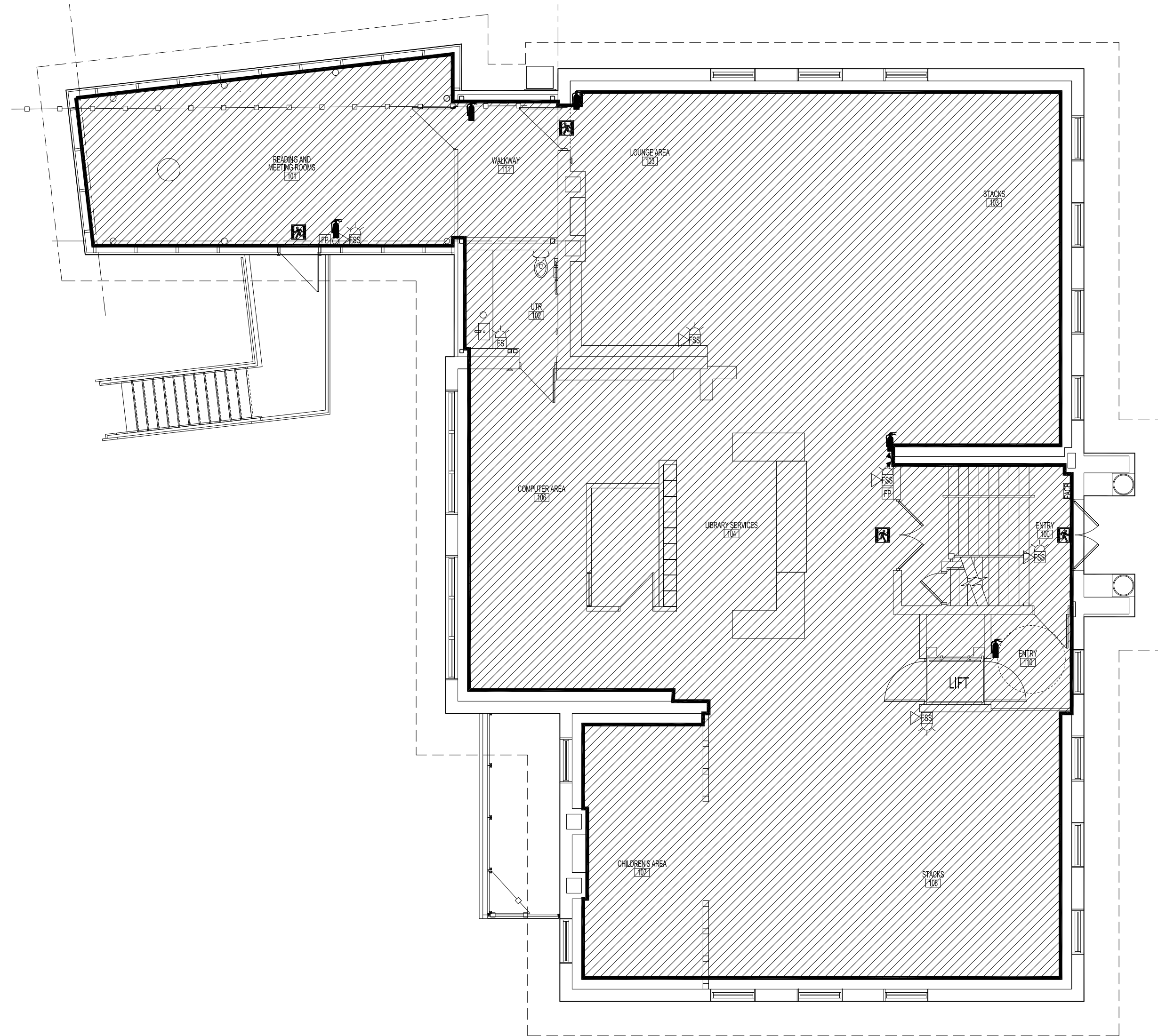
MAIN FLOOR PLAN SCALE: 1/8" = 1'-0"
